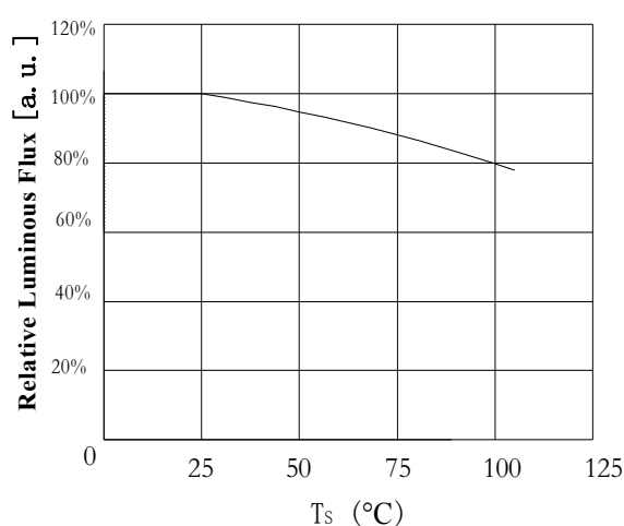
Case Temperature vs. Relative Luminous Flux 结点温度与相对流明曲线图 I_F = 150\text{mA}
