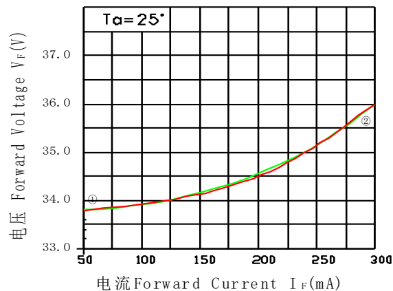
Forward Voltage vs. Forward Current 正向电压与正向电流曲线图
