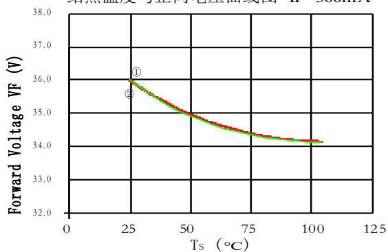
Case Temperature vs. Forward Voltage 结点温度与正向电压曲线图 I_F = 300\text{mA}
