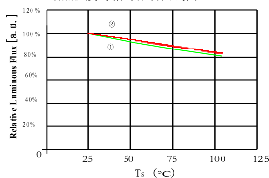
Case Temperature vs. Relative Luminous Flux 结点温度与相对流明曲线图 I_F = 300\text{mA}
