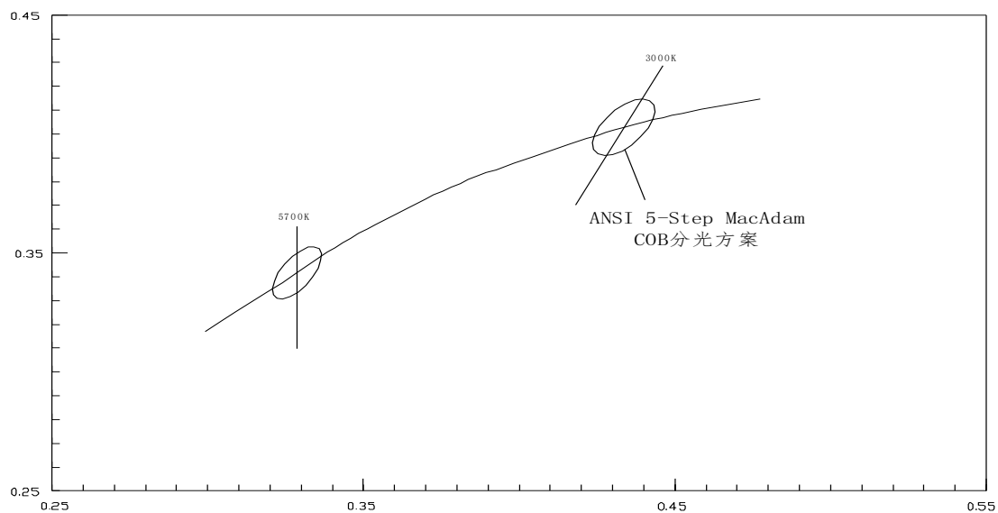
Chromaticity bins
