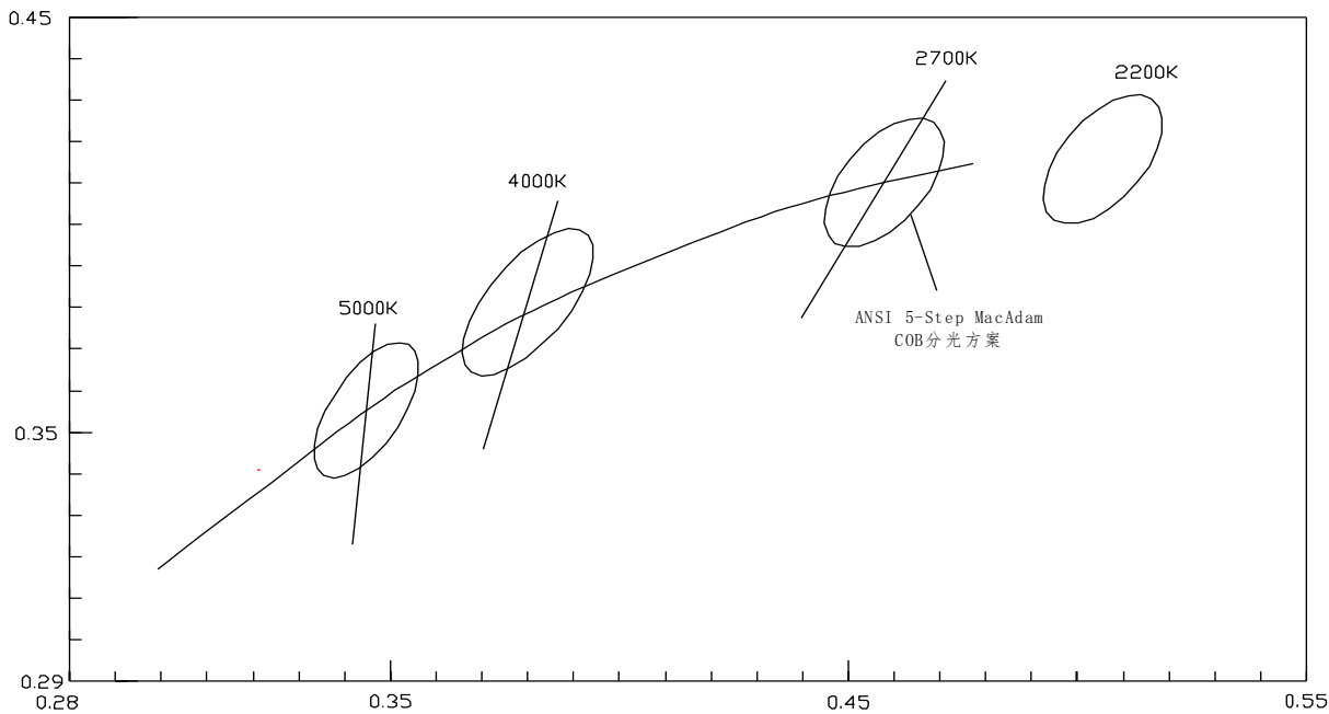
Chromaticity bins
