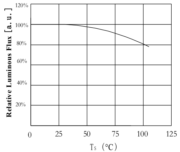
Case Temperature vs. Relative Luminous Flux 结点温度与相对流明曲线图 I_F = 600\text{mA}
