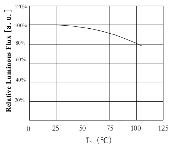
Case Temperature vs. Relative Luminous Flux 结点温度与相对照明曲线图 I_F = 850\text{mA}
