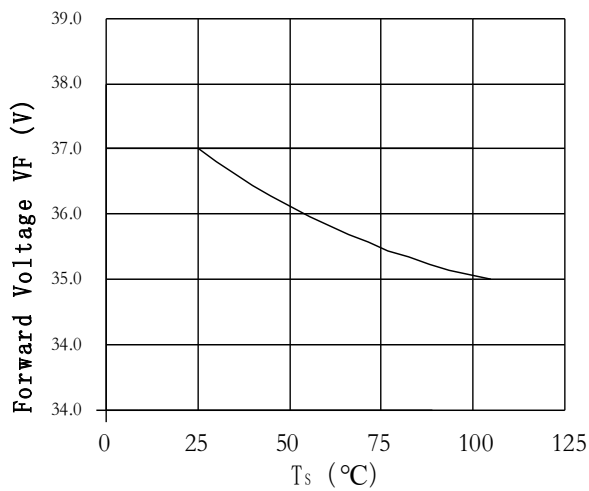
Case Temperature vs. Forward Voltage 结点温度与正向电压曲线图 I_F = 850\text{mA}
