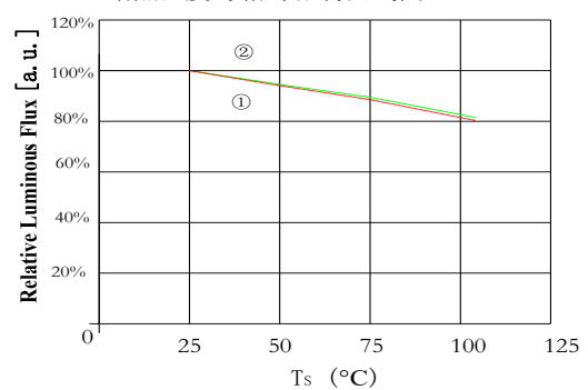
Case Temperature vs. Relative Luminous Flux 结点温度与相对流明曲线图 I_F=200\text{mA}
