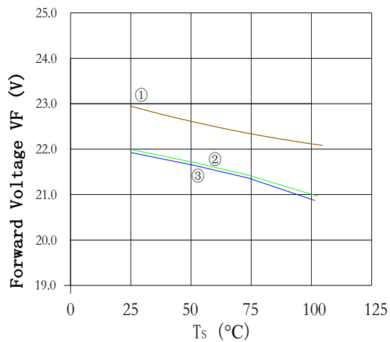
Case Temperature vs. Forward Voltage 结点温度与正向电压曲线图 I_F=200\text{mA}
