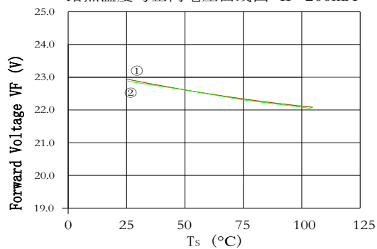
Case Temperature vs. Forward Voltage 结点温度与正向电压曲线图 I_F=200\text{mA}
