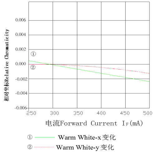
Warm White Current vs. Relative Chromaticity 暖白电流与相对坐标变化曲线图
