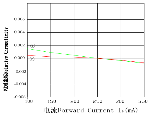
Warm White Current vs. Relative Chromaticity 暖白电流与相对坐标变化曲线图
