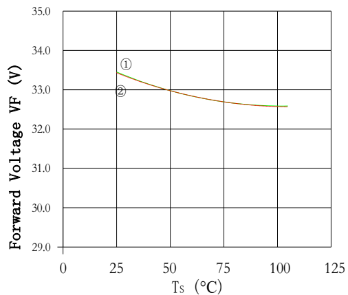
Case Temperature vs. Forward Voltage 结点温度与正向电压曲线图 I_F=600\text{mA}
