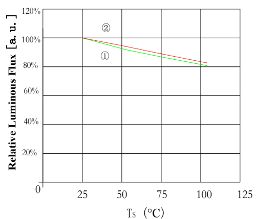
Case Temperature vs. Relative Luminous Flux 结点温度与相对光通量曲线图 I_F=600\text{mA}
