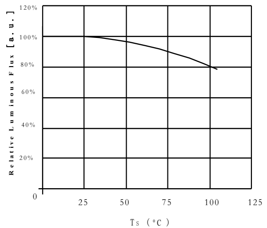
Case Temperature vs. Relative Luminous Flux 结点温度与相对流明曲线图 I F =1200mA
