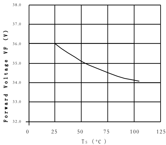
Case Temperature vs. Forward Voltage 结点温度与正向电压曲线图 I F =1200mA
